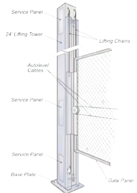
HydraLift™ Post
